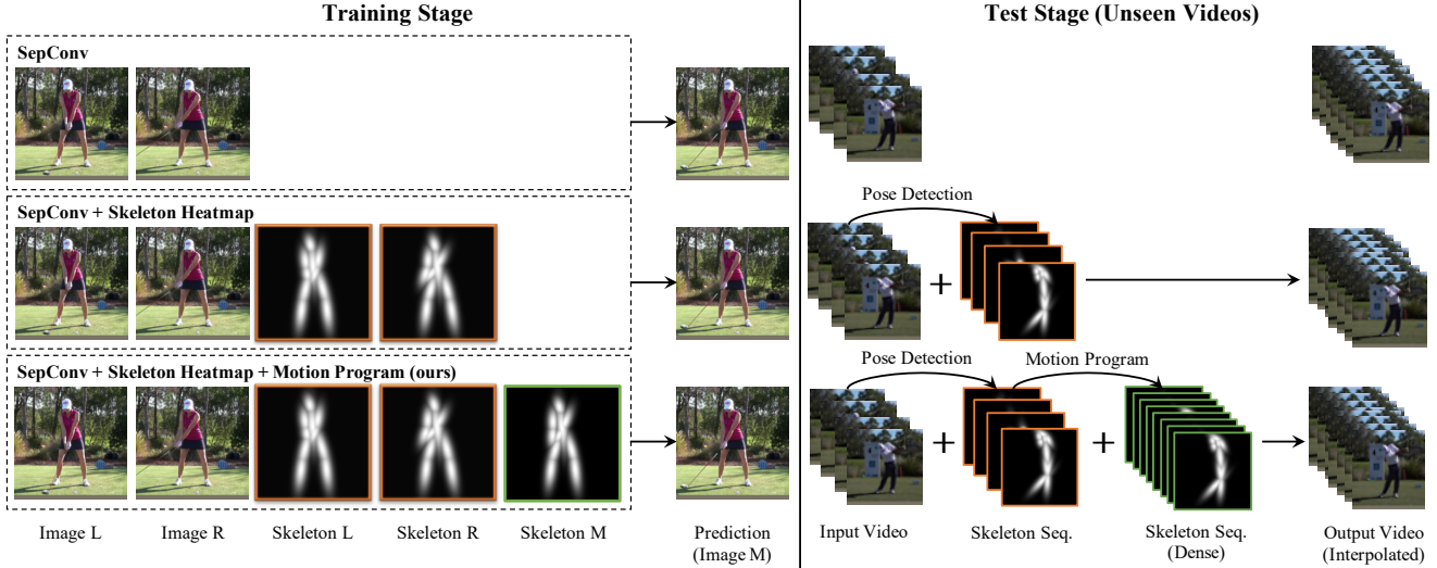
Figure 4. Evaluation of three video interpolation variants: Top row (SepConv [23]), middle row (SepConv w/ heatmaps) and bottom row (SepConv w/ programs) which is our model where poses for intermediate frames are supplied by motion programs. Middle row (SepConv w/ heatmaps) is evaluated as an ablation study.
