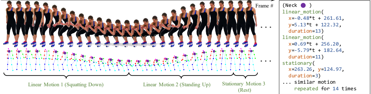
Figure 2. Examples of synthesized motion primitives. a) This golf swing has three primitives: back-swing, pause and down-swing. b) The squats sequence has a repeating subsequence of three similar primitives: squatting down, standing up and a brief rest in the standing pose.
