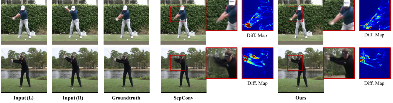
Figure 6. Qualitative results for 8x video interpolation. We observe that using program information results in uniformly higher image quality.
