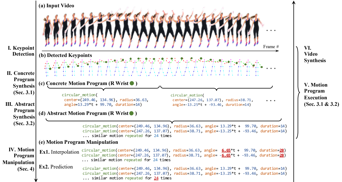
Figure 1. Overview of our hierarchical motion understanding framework. We start with low-level keypoints extracted from raw videos and build higher level motion understanding. Higher levels of abstraction consist of a sequence of motion primitives and their repetitive patterns. Similar motion in repetitive patterns are captured using a probabilistic for-loop body (refer Figure 3).
