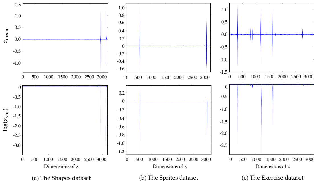
Figure 7-10: Statistics of latent vectors z_{\text{mean}} and z_{\text{logvar}} extracted from 1,000 image pairs from the Shapes, Sprites, and Exercise datasets, respectively. Each vertical line is for a single dimension in z . Although the z vector has 3,200 dimensions, only a small number of those have values deviating from the prior (mean 0, log-variance 0). This shows the system is learning to encode motion information in a compact way. Also, as the motion in the Exercise dataset is more complex, the system needs more bits for encoding (cf., Table 7.1).
