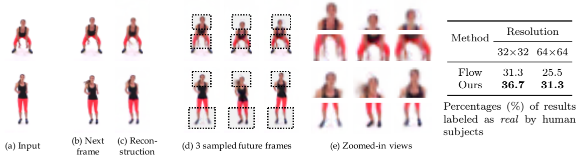
Figure 7-7: Results on the Exercise dataset. Left: We show input images (a), ground truth next frames (b), our reconstruction (c), three sampled future frames (d), and corresponding zoomed-in views (e). Right: Percentages (%) of synthesized results that were labeled as real by human subjects in two-way forced choices on Amazon Mechanical Turk, at resolution 32\times 32 and 64\times 64 . A perfect algorithm would achieve a percentage around 50%.
