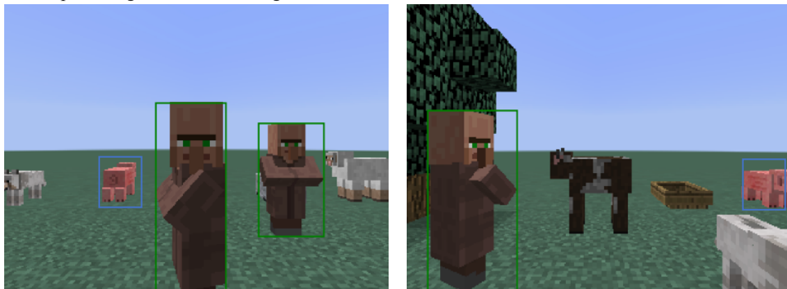
Figure B-7: Concepts learned on the Minecraft dataset
