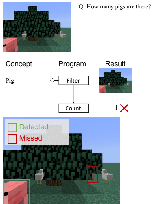
Figure B-4: Exemplar execution trace generated by our Neuro-Symbolic Concept Learner on the Minecraft reasoning dataset. Example A, B and C are successful execution. Example C demonstrates the semantics of the FilterMost operation. Example D shows a failure case: the detection model fails to detect a pig hiding behind the big tree.
