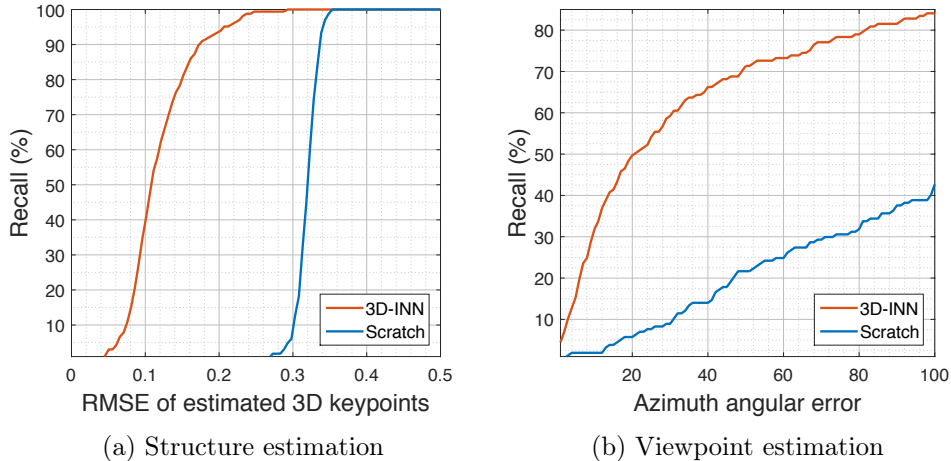
Figure 2-8: Evaluation the training paradigm on chairs from the IKEA dataset [Lim et al., 2013]. The network trained with our paradigm (3D-INN) is significantly better than the one trained from scratch on both 3D structure (a) and viewpoint estimation (b).
