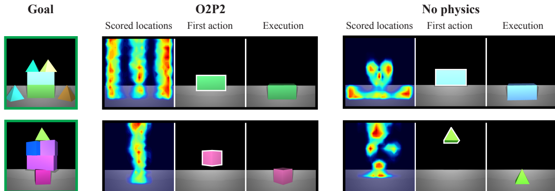
Figure 6-15: Heatmaps showing sampled action scores for the initial action given a goal block tower. O2P2’s scores reflect that the objects resting directly on the platform must be dropped first, and that they may be dropped from any height because they will fall to the ground. The No-physics ablation, on the other hand, does not implicitly represent that the blocks need to be dropped in a stable sequence of actions because it does not predict the blocks moving after being released.
