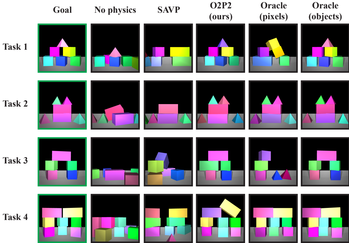
Figure 6-13: Qualitative results on building towers using planning. Given an image of the goal tower, we can use the learned object representations and predictive model in O2P2 for guiding a planner to place blocks in the world and recreate the configuration. We compare with an ablation, an object-agnostic video prediction model, and two ‘oracles’ with access to the ground-truth simulator.
