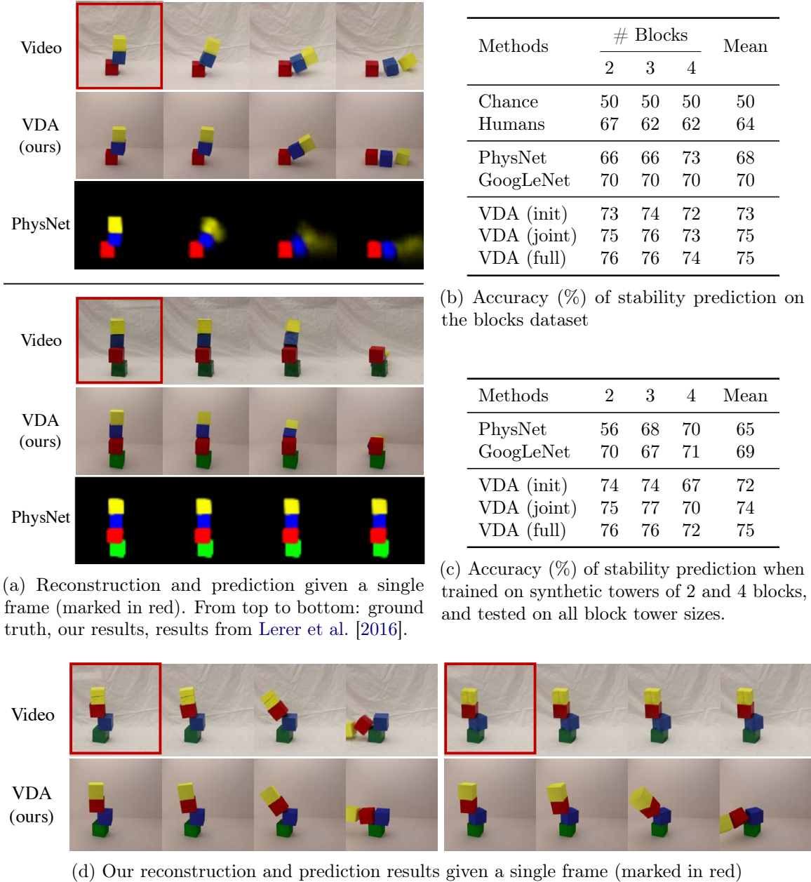
Figure 6-6: Results on the blocks dataset [Lerer et al., 2016]. For quantitative results (b), we compare three variants of our visual de-animation (VDA) model: perceptual module trained without fine-tuning (init), joint fine-tuning with REINFORCE (joint), and full model considering stability constraint (full). We also compare with PhysNet [Lerer et al., 2016] and GoogLeNet [Szegedy et al., 2015].
