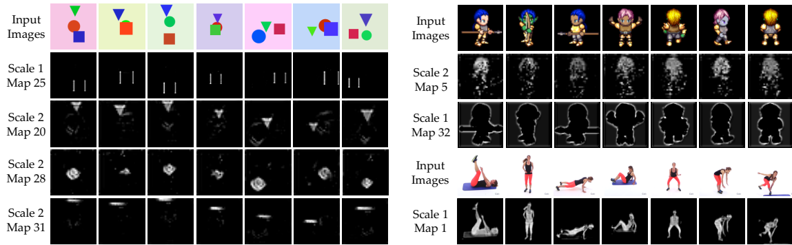
Figure 7-9: Learned layers on the Shapes dataset (left), the Sprites dataset (top right), and the Exercise dataset (bottom right). Our system is able to implicitly discover semantic structure from this self-supervised task. On the Shapes dataset, it learns to detect circles and triangles; it also detects vertical boundaries of squares, as squares always move horizontally. On the Exercise dataset, it learns to respond to only humans, not the carpet below them, as the carpet never moves.
