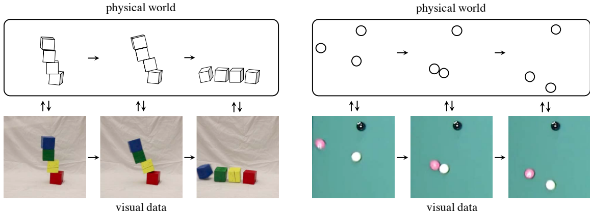
Figure 6-1: Visual de-animation —we would like to recover the physical world representation behind the visual input, and combine it with generative physics simulation and rendering engines.
