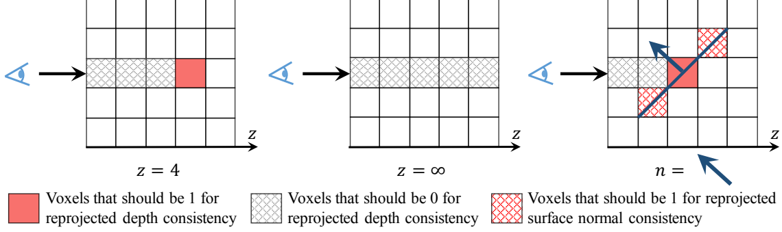
Figure 3-5: Reprojection consistency between 2.5D sketches and 3D shape. Left and middle: the criteria for depths and silhouettes; right: the criterion for surface normals. See Section 3.4.3 for details.
