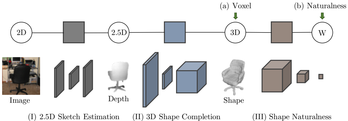
Figure 3-9: ShapeHD contains three components: (I) a 2.5D sketch estimator that predicts depth, surface normal and silhouette images from a single image; (II) a 3D shape completion module that regresses 3D shapes from silhouette-masked depth and surface normal images; (III) an adversarially pretrained convolutional net that serves as the naturalness loss function. While fine-tuning the 3D shape completion net, we use two losses: a supervised loss on the output shape, and a naturalness loss offered by the pretrained discriminator.
