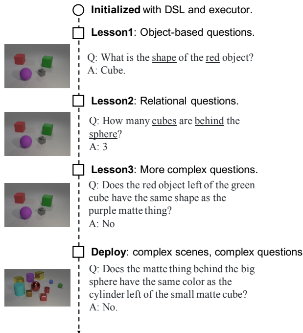
Figure 8-7: A. Demonstration of the curriculum learning of visual concepts, words, and semantic parsing of sentences by watching images and reading paired questions and answers. Scenes and questions of different complexities are illustrated to the learner in an incremental manner. B. Illustration of our neuro-symbolic inference model for VQA. The perception module begins with parsing visual scenes into object-based deep representations, while the semantic parser parse sentences into executable programs. A symbolic execution process bridges two modules.
