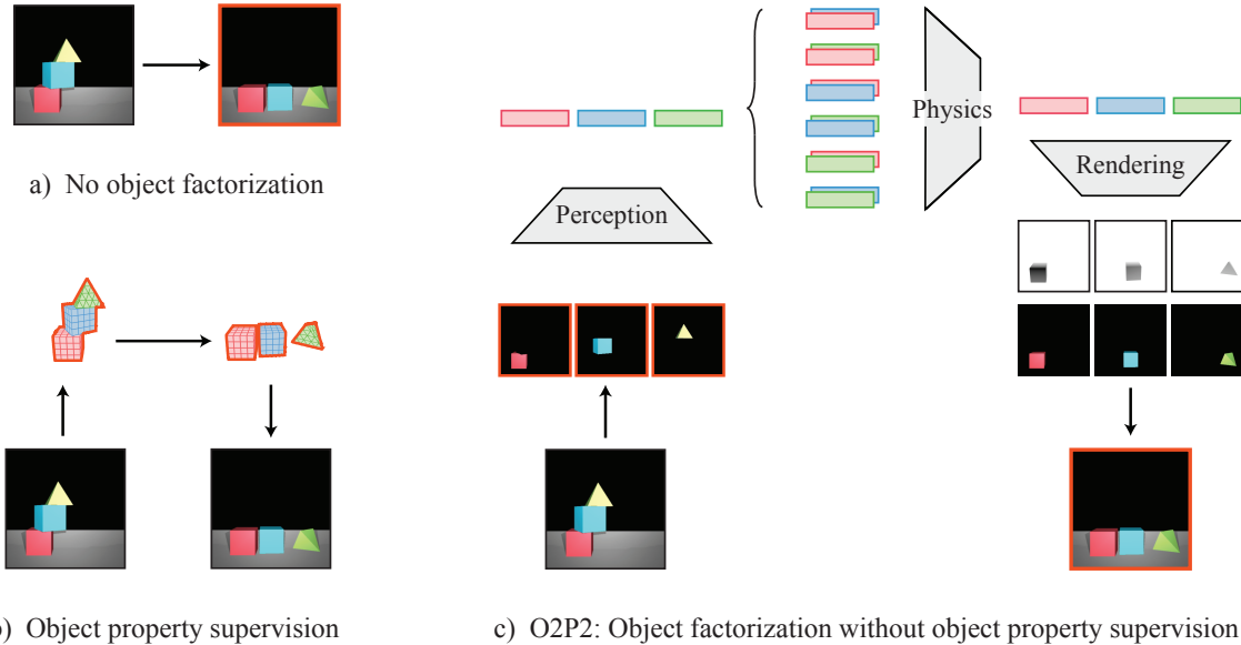
Figure 6-12: We divide physical understanding tasks into three distinct paradigms. (a) The first approach makes the fewest assumptions, posing prediction tasks as an instance of image-to-image translation. (b) The second uses ground-truth labels of object properties to supervise a learning algorithm that can map to the space of a traditional or learned physics engine. (c) O2P2, like (b), employs an object factorization and the functional structure of a physics engine, but like (a), does not assume access to supervision of object properties. Without object-level supervision, we must jointly learn a perception function to map from images to objects, a physics engine to simulate a collection of objects, and a rendering engine to map a set of objects back to a single composite image prediction. In all three approaches, we highlight the key supervision in orange .
