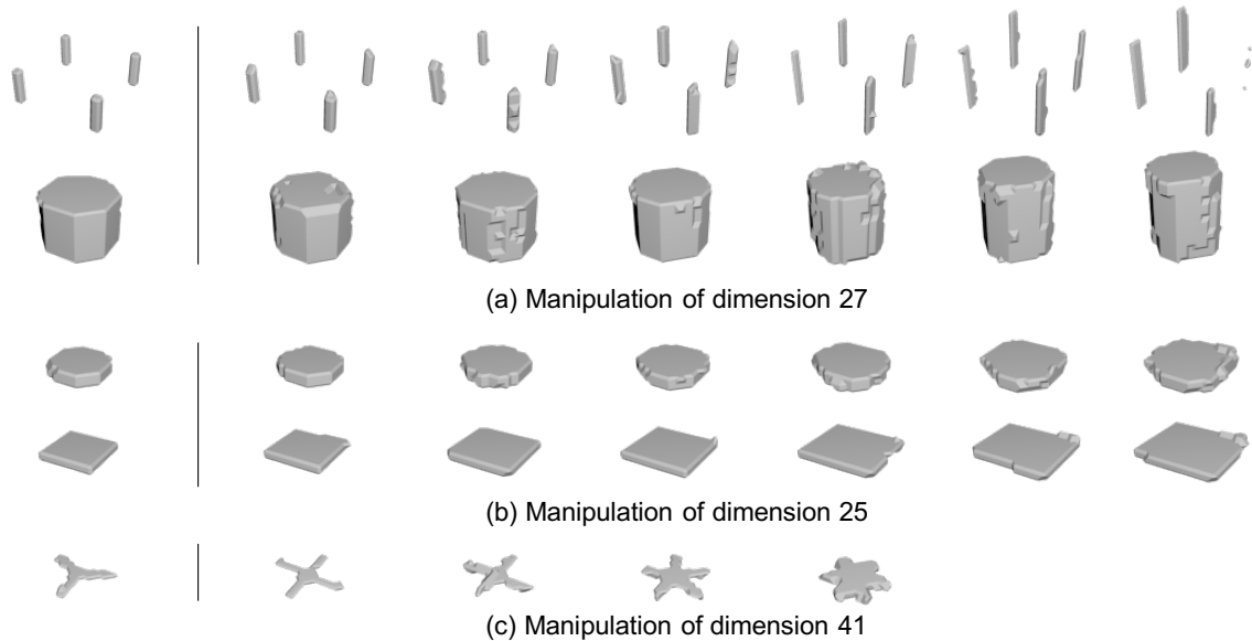
Figure 9-8: We visualize the effect of manipulating individual dimensions in the intermediate representation of neural program executor. For example, dimension 27 corresponds to the height of primitives, dimension 25 to the radius of primitives, and dimension 41 to the times of primitive repetition.
