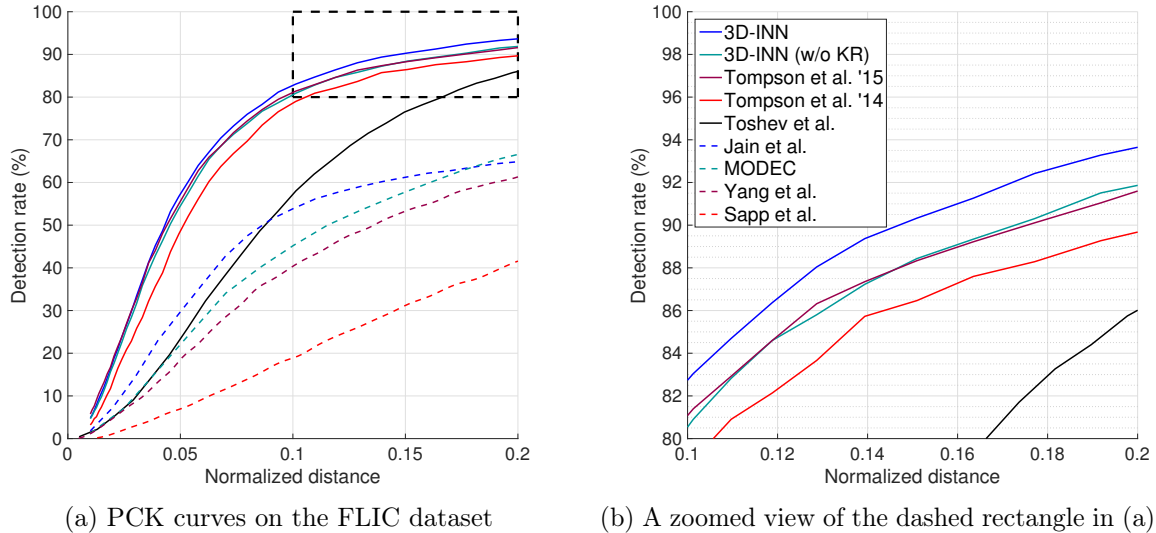
Figure 2-5: Results on human keypoint estimation. (a) PCK curves on the FLIC dataset [Sapp and Taskar, 2013]. 3D-INN performs consistently better than other methods. Without keypoint refinement, it is comparable to Tompson et al. [2015]. (b) A zoomed view of the dashed rectangle in (a).
