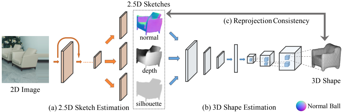
Figure 3-4: Our model (MarrNet) has three major components: (a) 2.5D sketch estimation, (b) 3D shape estimation, and (c) a loss function for reprojection consistency. MarrNet first recovers object normal, depth, and silhouette images from an RGB image. It then regresses the 3D shape from the 2.5D sketches. In both steps, it uses an encoding-decoding network. It finally employs a reprojection consistency loss to ensure the estimated 3D shape aligns with the 2.5D sketches. The entire framework can be trained end-to-end.
