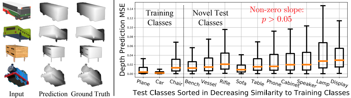
Figure 3-14: Results on depth prediction. Left: Our single-view depth estimator, trained on cars, chairs, and airplanes, generalizes to novel classes: buses, trains, and tables. Right: As the novel test class gets increasingly dissimilar to the training classes (left to right), depth prediction does not show statistically significant degradation ( p > 0.05 ).
