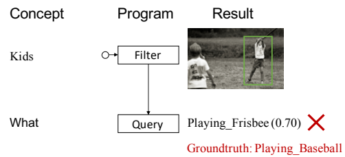
Figure B-5: Exemplar execution trace generated by our Neuro-Symbolic Concept Learner on the VQS dataset. Execution traces A and B shown in the figure leads to the correct answer to the question. Our model effectively learns visual concepts from data. The symbolic reasoning process brings transparent execution trace and can easily handle quantities (e.g., object counting in Example A). In Example C, although NS-CL answers the question correctly, it locates the wrong object during reasoning: a dish instead of the cake. In Example D, our model misclassifies the sport as frisbee.
