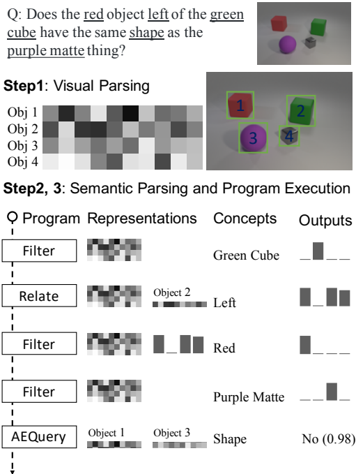
Figure 8-7: A. Demonstration of the curriculum learning of visual concepts, words, and semantic parsing of sentences by watching images and reading paired questions and answers. Scenes and questions of different complexities are illustrated to the learner in an incremental manner. B. Illustration of our neuro-symbolic inference model for VQA. The perception module begins with parsing visual scenes into object-based deep representations, while the semantic parser parse sentences into executable programs. A symbolic execution process bridges two modules.
