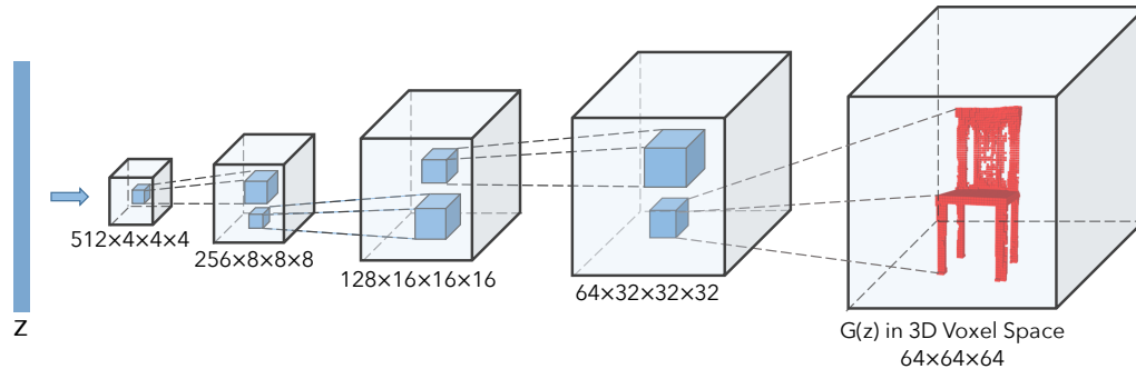
Figure 3-6: The generator in 3D-GAN. The discriminator mostly mirrors the generator.
