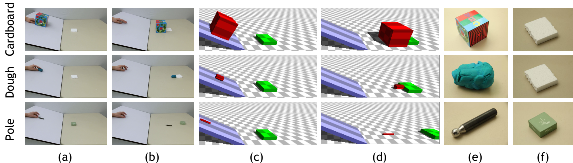
Figure 5-5: Simulation results. Each row represents one video in the data: (a) the first frame of the video, (b) the last frame of the video, (c) the first frame of the simulated scene generated by Bullet, (d) the last frame of the simulated scene, (e) the estimated object with larger mass, (f) the estimated object with larger friction coefficient.
