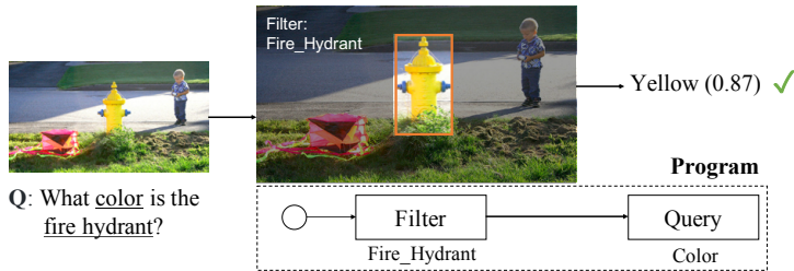
Figure 8-9: Demo from the VQS dataset. An example image-question pair from the VQS dataset and the corresponding execution trace of NS-CL.
