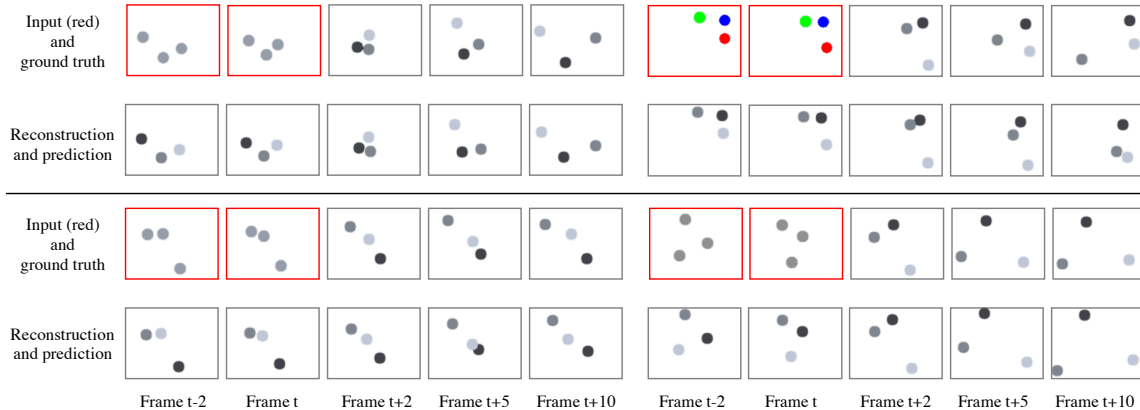
Figure 6-4: Qualitative results on the billiard videos , comparing ground truth videos with our predictions. We show two of three input frames (in red) due to space constraints. Left: balls share appearance and physics (I), where our framework learns to discover objects and simulate scene dynamics. Top right: balls have different appearance and physics (II), where our model learns to associate appearance with physics and simulate collisions. It learns that the green ball should move further than the heavier blue ball after the collision. Bottom right: balls share appearance but have different frictions (III), where our model learns to associate motion with friction. It realizes from three input frames that the right-most ball in the first frame has a large friction coefficient and will stop before the other balls.
