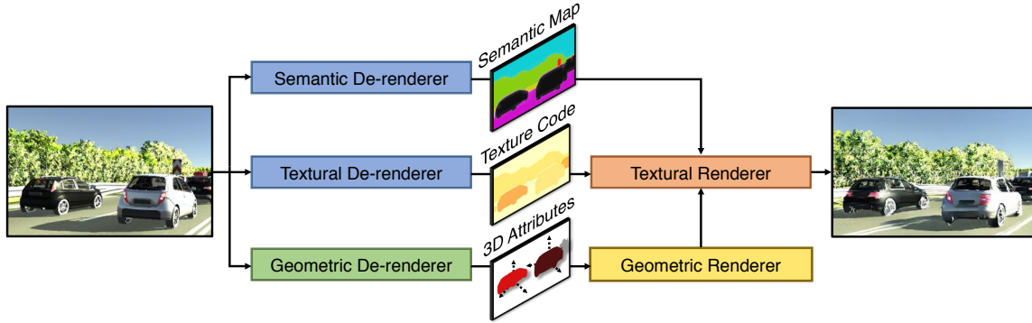
Figure 4-6: Overview of 3D-SDN. The de-renderer (encoder) consists of a semantic-, a textural- and a geometric branch. The textural renderer and geometric renderer then learn to reconstruct the original image from the representations obtained by the encoder modules.
