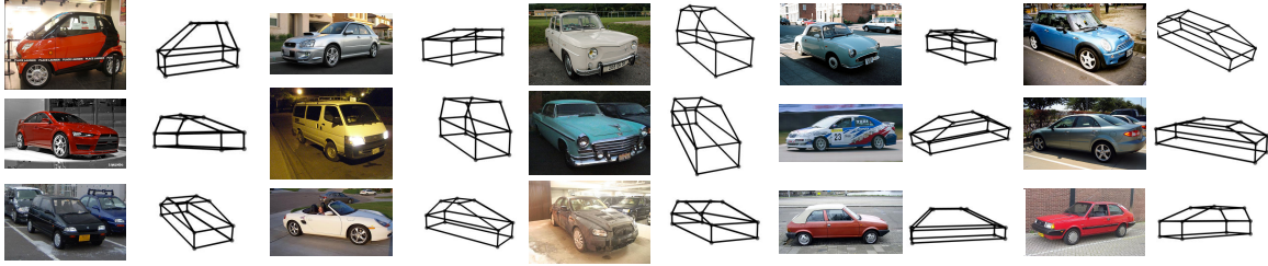
Figure 2-11: Car structure estimation on images from the PASCAL 3D+ dataset [Xiang et al., 2014]
