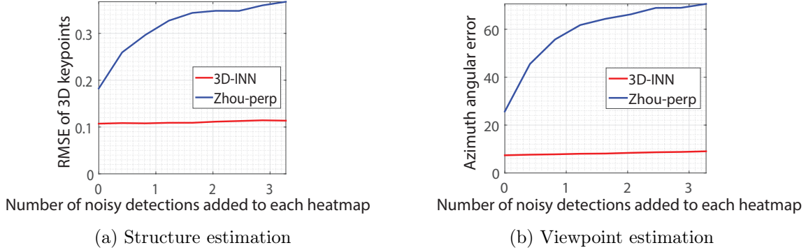
Figure 2-7: Plots comparing our method against an analytical solution on synthetic heatmaps. (a) The accuracy of 3D structure estimation; (b) The accuracy of 3D viewpoint estimation.
