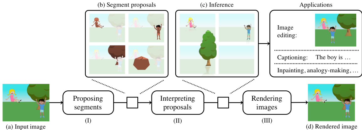
Figure 4-5: Our neural scene de-rendering framework consists of three component. Given an input image, it first generates a number of segment proposals (Stage I). It then tries to interpret if there is an object in the each proposal, and if so what its properties are (Stage II). Eventually, these inference results are integrated and sent to a graphics engine for rendering, so that the original image can be reconstructed (Stage III). We have supervision on both the latent representation space and the image space. Also note that the latent representations have wide applications including image editing, captioning, etc.
