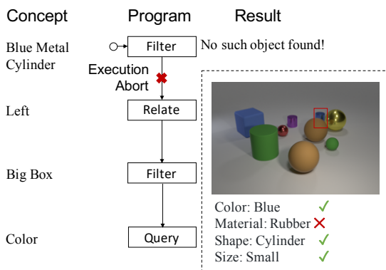
Figure B-3: Exemplar execution trace generated by our Neuro-Symbolic Concept Learner on the CLEVR dataset . Example A and B are successful executions that generate correct answers. In example C, the execution aborts at the first operator. To inspect the reason why the execution engine fails to find the corresponding object, we can read out the visual representation of the object, and locate the error source as the misclassification of the object material. Example D shows how our symbolic execution engine can detect invalid or ambiguous programs during the execution by performing sanity checks.
