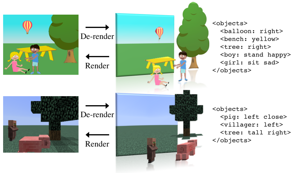
Figure 4-1: Our goal is to interpret an image in a holistic way. Assuming an image is rendered by a graphics engine on an indefinite length input, we aim to recover the input so that the the exact image can be reconstructed and manipulated. Here we show a simplified version of the XML we use.
