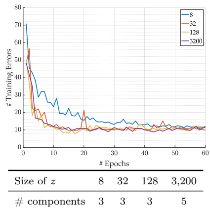
Figure 7-12: Ablation study on the size of z . Our model automatically discovers the underlying dimension of the motion (the number of dominating PCA components) in the Shapes dataset. When we shrink the size of z , the convergence gets a little slower (especially when z has only 8 dimensions), but the results are essentially the same.
