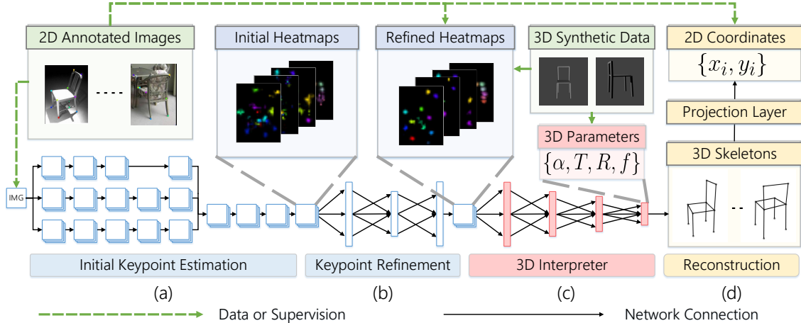
Figure 2-4: Architecture of 3D-INN . 3D-INN takes a single image as input and reconstructs the detailed 3D structure of the object in the image (e.g., human, chair, etc.). The network is trained independently for each category, and here we use chairs as an example. (a) Estimating 2D keypoint heatmaps with a multi-scale CNN. (b) Refining keypoint locations by considering the structural constraints between keypoints. This is implicitly enforced with an information bottleneck and yields cleaner heatmaps. (c) Recovered 3D structural and camera parameters \{\alpha, T, R, f\} . (d) The projection layer maps reconstructed 3D skeletons back to 2D keypoint coordinates.
