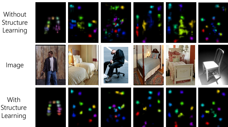
Fig. 5: 2D keypoint predictions from a single image, where each color corresponds to a keypoint. The keypoint refinement step cleans up false positives and produces more regulated predictions.
