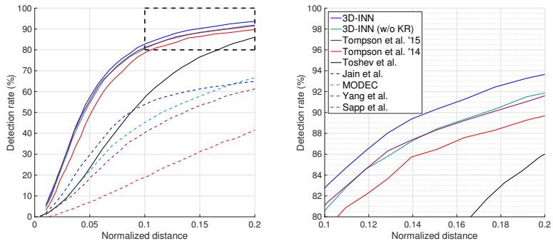
Fig. 4: PCK curves on the FLIC dataset. 3D-INN performs consistently better than other methods. Without keypoint refinement, it is comparable to Tompson et al. [44]. A zoomed view of the dashed rectangle is shown on the right.
