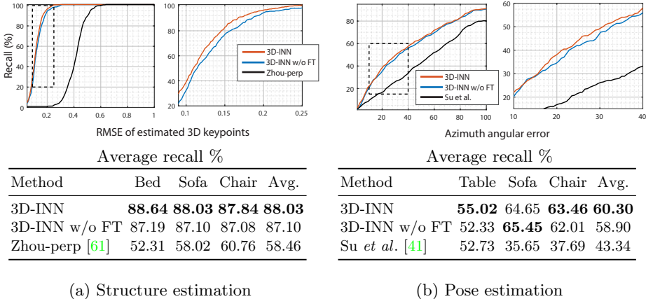
Fig. 7: Evaluation on the IKEA dataset [25]. (a) The accuracy of structure estimation. RMSE-Recall curved is shown in the first row, and zoomed-views of the dashed rectangular regions are shown on the right. The third row shows the average recall on all thresholds. (b) The accuracy of pose estimation.
