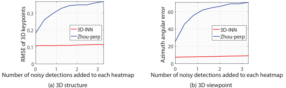
Fig. 6: Plots comparing our method against an analytic solution on synthetic heatmap. (a) The accuracy of 3D structure estimation; (b) The accuracy of 3D viewpoint estimation.
