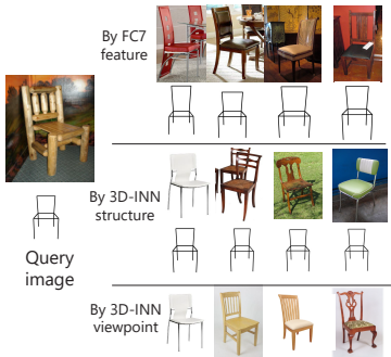
Fig. 10: Retrieval results in different feature spaces. 3D-INN helps to retrieve objects with similar 3D structures or similar viewpoints.
